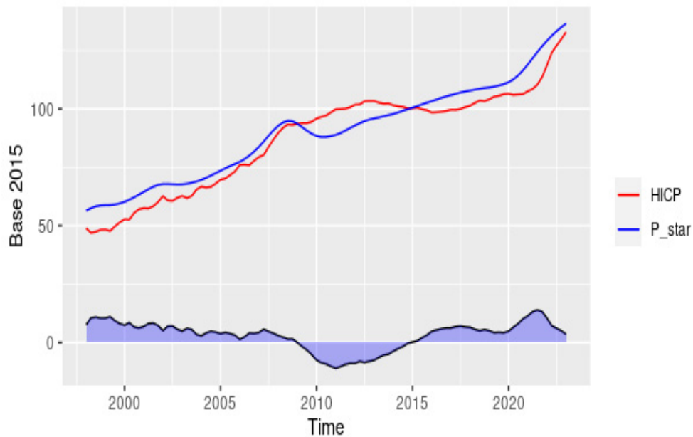
Figure 7. Price Gap
