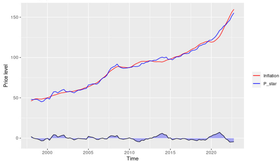
Figure 4. Price Gap
